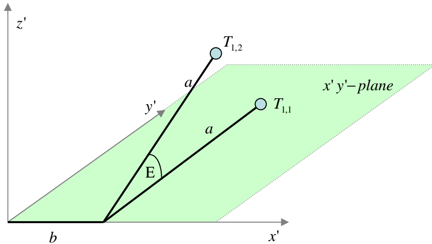
Figure 2: Point definition
