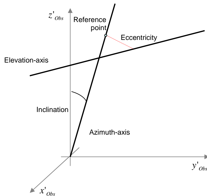
Figure 1: Restrictions (eccentricity and inclination), for clearness shown in the coordinate system x'_{Obs} , y'_{Obs} , z'_{Obs} , which emantes from the observation system x_{Obs} , y_{Obs} , z_{Obs} by translation
